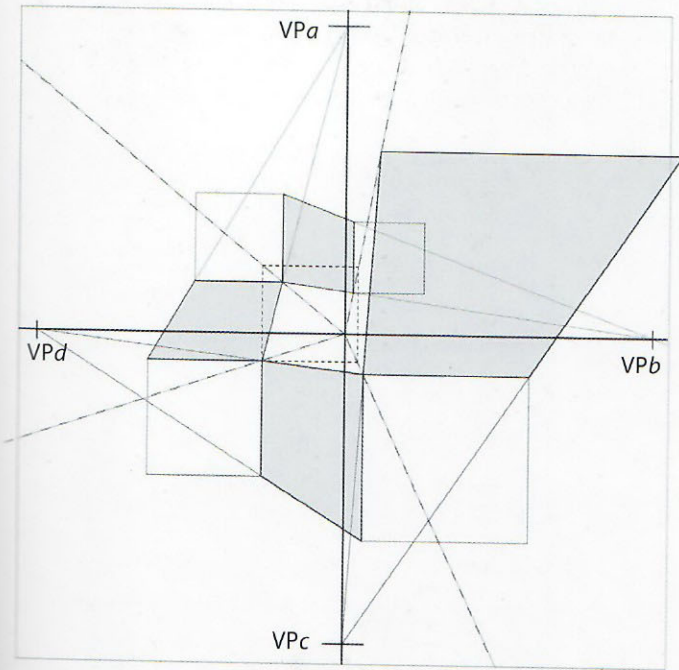
Fig. 7.21: Here are the four inclined planes going in four different directions.
