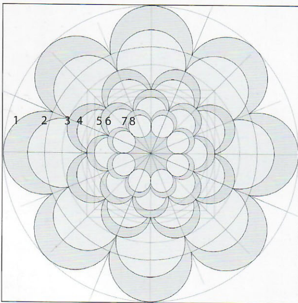
Fig. 8.56: The top view outline of level 1 also corresponds to the base of the building; the top view of section 2 also corresponds to its base, and so on.
